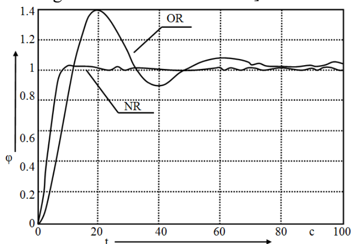
2-rasm. Real jarayonning o'zgarib borish egri chiziqlari.
