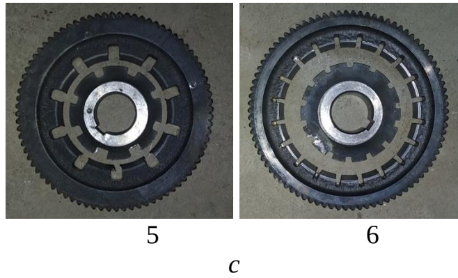
a-slope angle 15°; b-slope angle 17°; c- slope angle 19°; 1, 3, 5 intermediate shaft gear wheel; 2, 4, 6-last shaft gear wheel.
